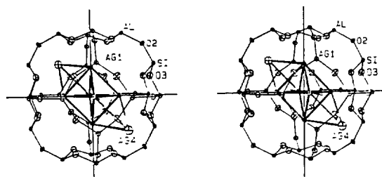
Figure 4. A stereoview of a sodalite unit containing an Ag 6 molecule complexed to two Ag + ions is shown. Ellipsoids of 20% probability are used.
