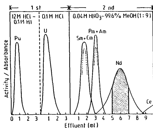
Fig. 2. Anion Exchange Chromatogram with 12 M HCl-0.1 M HI, 0.1 M HCl and Methanolic- HNO 3 Eluent
