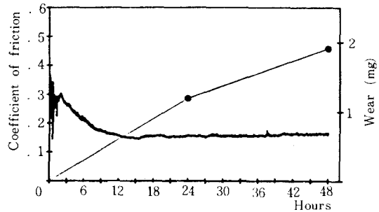
Fig. 8. Friction coefficient and wear rate of the composite tested in normal direction. (normal load = 9.6N, sliding speed = 2.5m/s)
