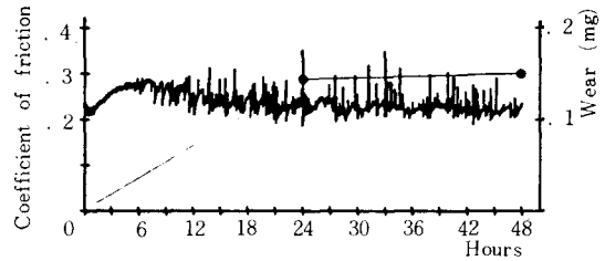
Fig. 3. Friction coefficient and wear of the composite tested in transverse direction (normal load =49N, sliding speed =0.5m/s)
