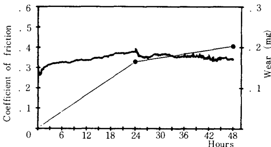
Fig. 2. Friction coefficient and wear of the composite tested in longitudinal direction (normal load =49 N, sliding speed =0.5m/s)
