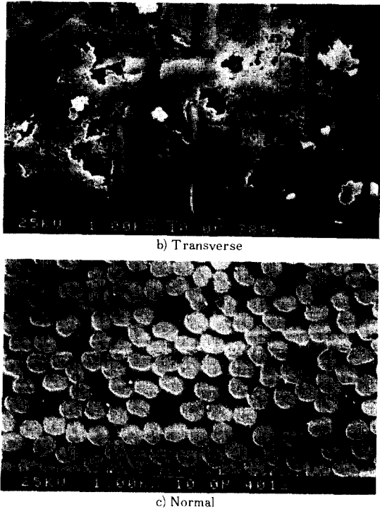
Fig. 5. Micrographs of the wear track for different fiber orientations. (normal load = 49N, sliding speed = 0.5m/s)
