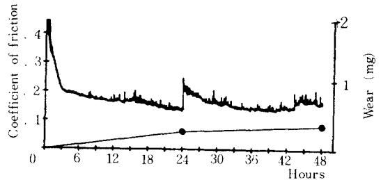
Fig. 7. Friction coefficient and wear of the composite tested in transverse direction. (normal load = 19.6N, sliding speed = 2.5m/s)
