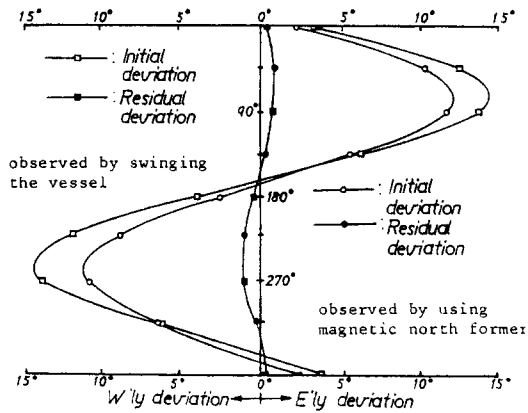
Fig. 5. Initial deviation and residual deviation curves by using magnetic north former at ship's heading 000° and by observing the bearing of a distant object.
