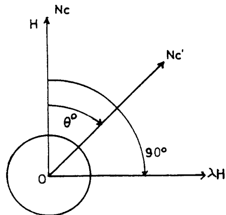
Fig. 2. Adjusting the magnetic fields by both A and B arms of magnetic north former
