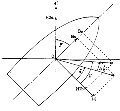
Fig. 7. The effect of inaccurate compensation for the initial directive force.
