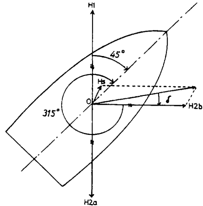
Fig. 4. Deviaton at ship's heading 315°, simulated by the magnetic north former.
