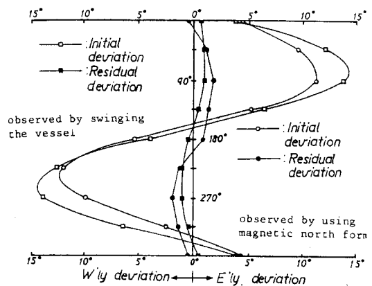
Fig. 6. Initial deviation and residual deviation curves by using magnetic north former at ship's heading 045° and by observing the bearings of a distant object.
