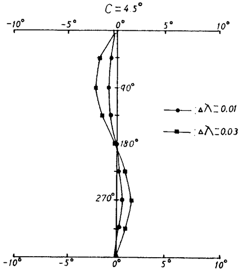
Fig. 10. The error contained in the coefficient C when the directive force is over-compensated by 0.01 or 0.03.
