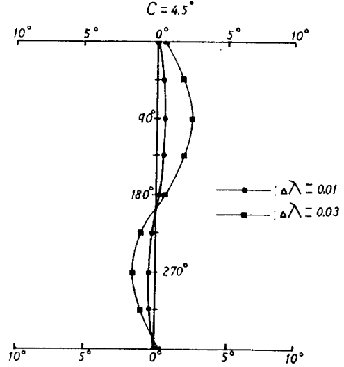
Fig. 11 The error contained in the coefficient C when the directive force is short-compensated by 0.01 or 0.03.
