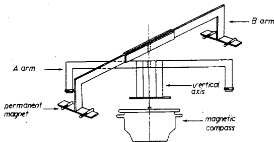
Fig. 1. Magnetic north former.
