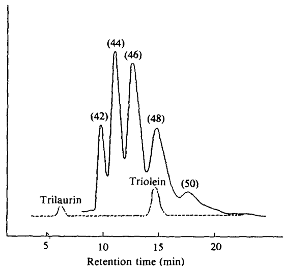
Fig. 1. HPLC chromatogram of sesame oil (Chonnam). Numbers in parenthesis indicate partition number (PN).
