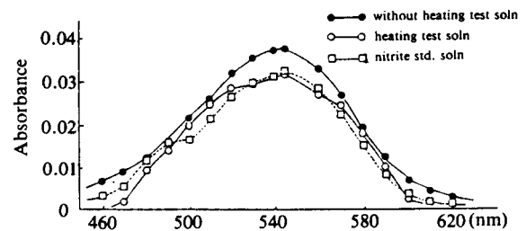
Fig. 2. Absorbance spectra of test solution extracted with and without heating at 80°C for 2 hrs. Test solution was added HgCl 2 .
