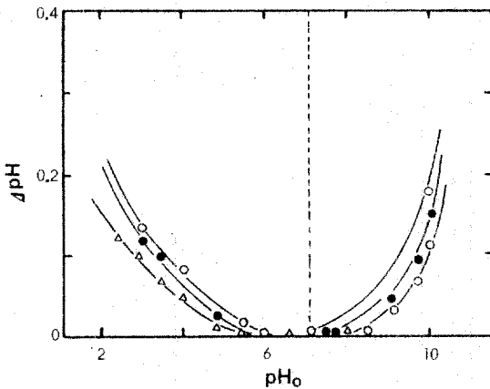
Fig. 3. Determination of isoelectric point of 2-(dimethylalkylammonio) propanoates at 25°C.
