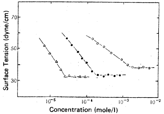
Fig. 6. Surface tension of (dimethyl alkyl ammonio) ethanoates.
