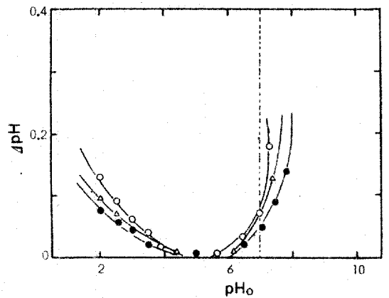
Fig. 4. Determination of isoelectric point of 2-(dimethylalkylammonio)-3-phenylpropanoates at 25°C.
