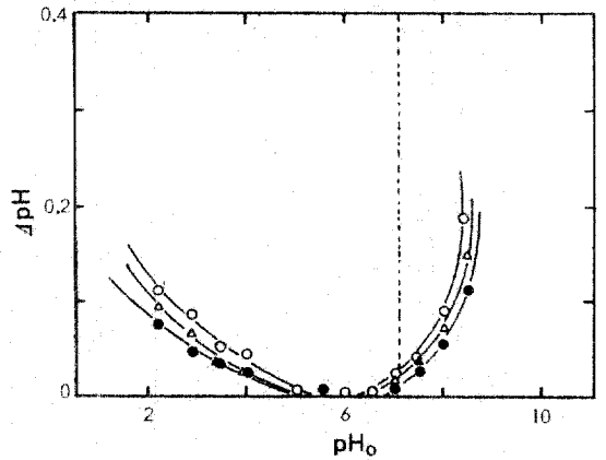
Fig. 2. Determination of isoelectric point of (dimethylalkylammonio) ethanoates at 25°C.
