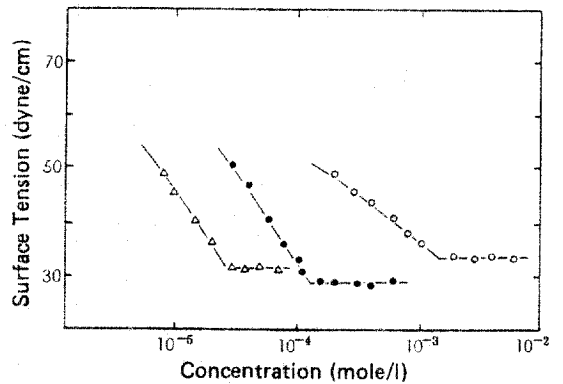
Fig. 7. Surface tension of 2-(dimethyl alkyl ammonio) propanoates.
