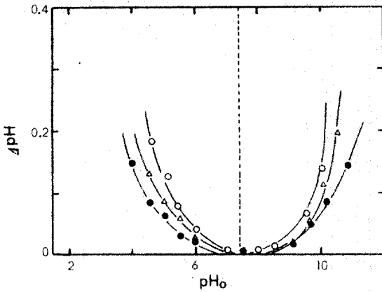
Fig. 1. Determination of isoelectric point of 2-(trimethylammonio) alkanooates, at 25°C.
