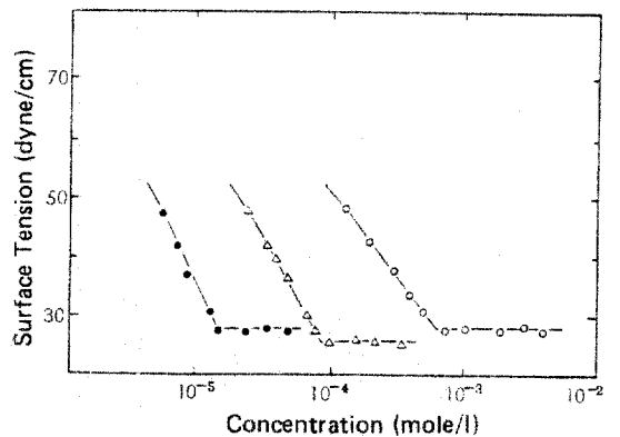
Fig. 8. Surface tension of 2-(dimethyl alkyl ammonio)-3-phenylpropanoates.
