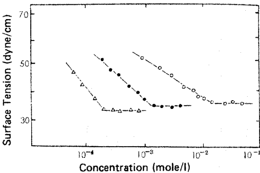
Fig. 5. Surface tension of 2-(trimethylammonio)alkanoates.
