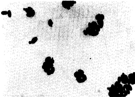
Fig. 4. Morphological appearance of Kluyveromyces fragilis (x 1500).
