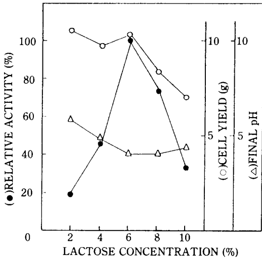
Fig. 1. Effect of lactose concentration on the Formation of Beta-galactosidase
