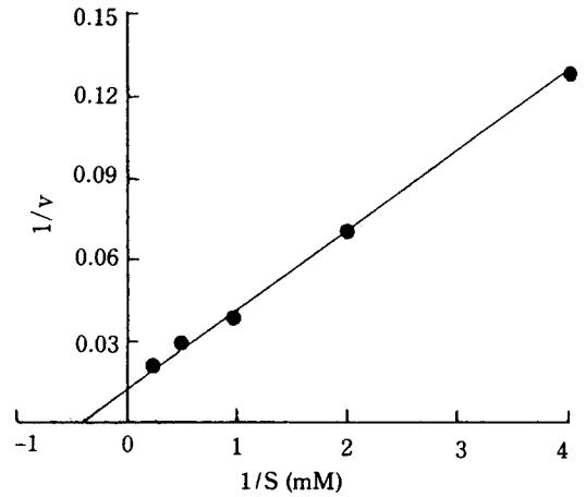
Fig. 9. Lineweaver-Burk double reciprocal plot for determination of the Michaelis constant for the hydrolysis of ONPG.
