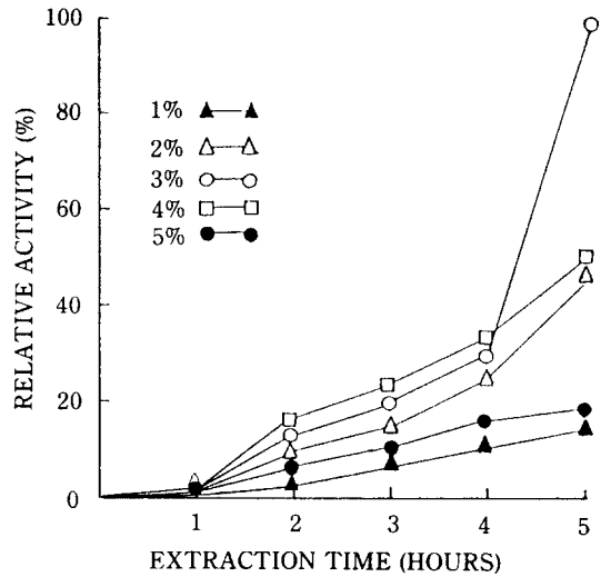
Fig. 3. Effect of time and toluene concentration on the extraction of Beta-galactosidase.
