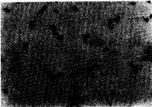
Fig. 5. Morphological appearance of Kluyveromyces fragilis after toluene treatment (x 1500).
