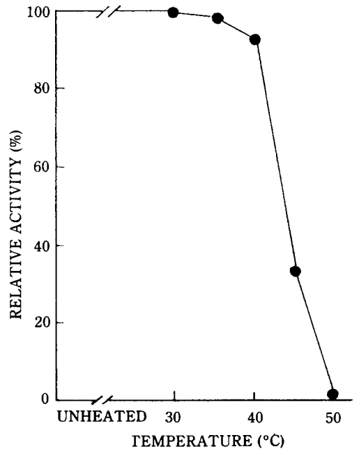
Fig. 7. Effect of heat treatment on enzyme activity.
