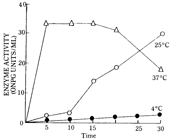
Fig. 2. Effect of time and temperature on extraction of Beta-galactosidase by toluene treatment.
