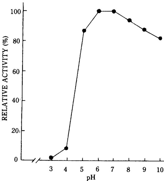
Fig. 8. Effect of pH on the stability of Beta-galactosidase.
