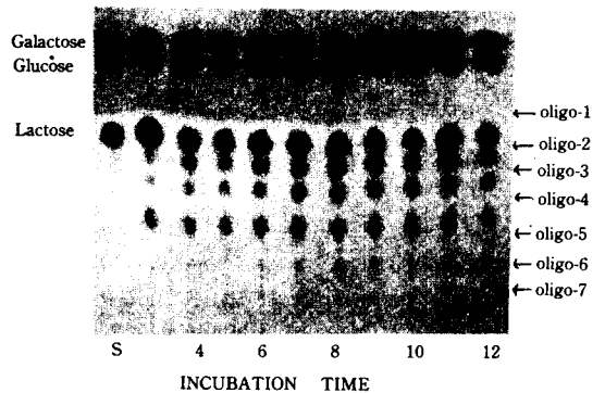
Fig. 10. Paper Chromatogram of Lactose Hydrolyzates. 40% of Lactose solution in 0.05M phosphate Buffer, pH 7.0, was hydrolyzed at 45°C. S, Stander.
