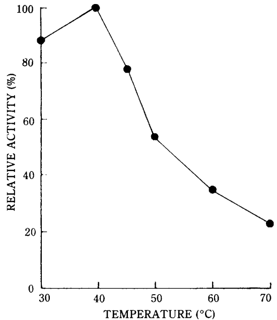
Fig. 6. Effect of temperature on enzyme activity.
