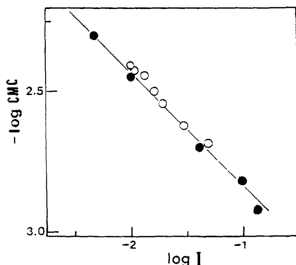
Figure 4. The dependence of the critical micelle concentration of NaDC on the ionic strength of medium. The ionic strength was adjusted with NaCl in 0.001 M tris buffer (O) or with phosphate buffer (●).
