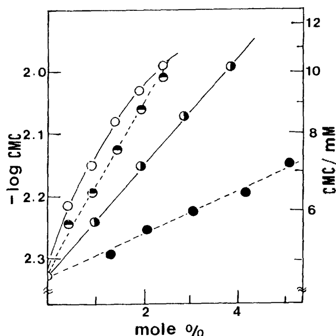
Figure 3. The dependence of the critical micelle concentration of NaDC on the proportion of amides: -O-, N -methylacetamide; -●-, DMF; -●-, acetamide; -●-, formamide.
