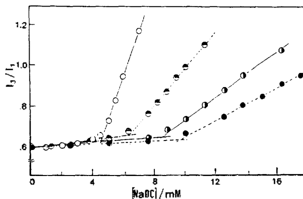
Figure 2. The variations of I_3/I_1 of pyrene fluorescence as functions of NaDC concentration. The proportions of DMF in solvent were 0(O), 1(O), 2(O) and 2.5(O) mole %.
