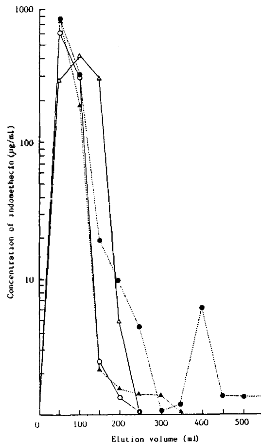
Figure 3. In vitro release of indomethacin from monolithic device during burst period in continuous elution system. \Delta - \Delta 100:0 glutamic acid: leucine, \blacktriangle - \blacktriangle ; 70:30, \circ - \circ ; 50:50, \odot - \odot ; 20:80, \bullet - \bullet ; 10:90.
