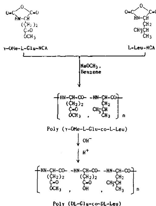
Figure 1. Preparation of copolypeptides of glutamic acid and leucine.
