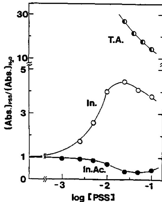
Figure 2. Variations in absorbance at 390 nm of 5 mM indole derivatives-5 mM MV** mixtures with PSS concentration. The pH of indole acetate was 7, and that of tryptamine was 3. Temperature of indole was 35°C, and others were 25°C.
