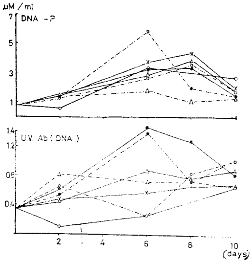
Fig. 6. Changes in amount of total-P and UV absorbing material in DNA fraction treating with various kinds of sugar as carbon source.
