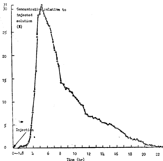
Fig. 3. Recovery curve for 51 Cr-EDTA in steel sawdust.
