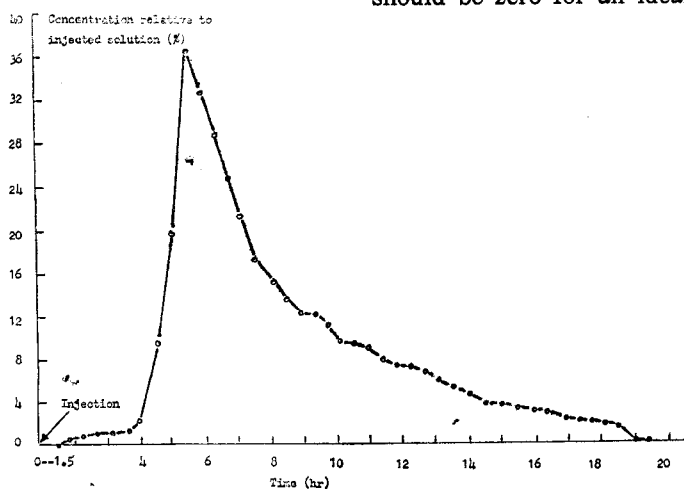
Fig. 4. Recovery curve for 51 Cr-DTPA in quartz sand.
