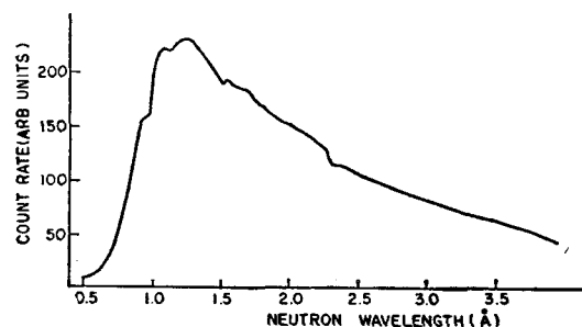
Fig. 3. The Observed Count Rate of Neutrons Reflected by the Monochromator.
