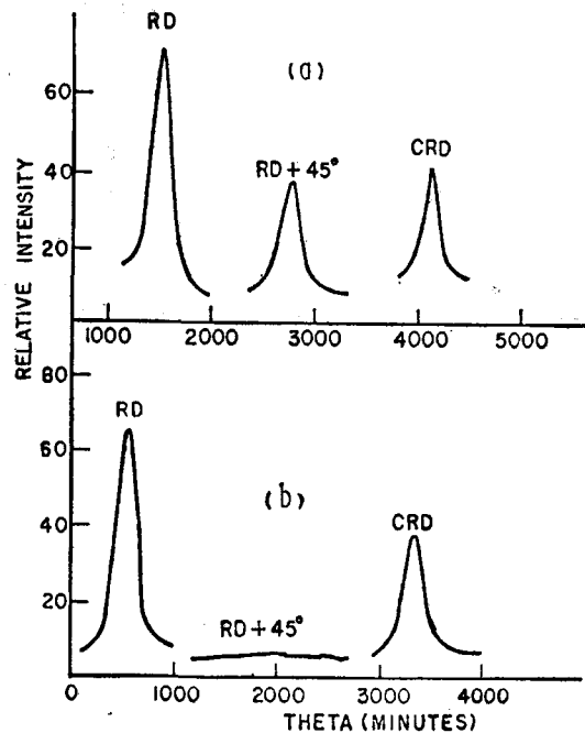
Fig. 8. The rocking curves of series C.
