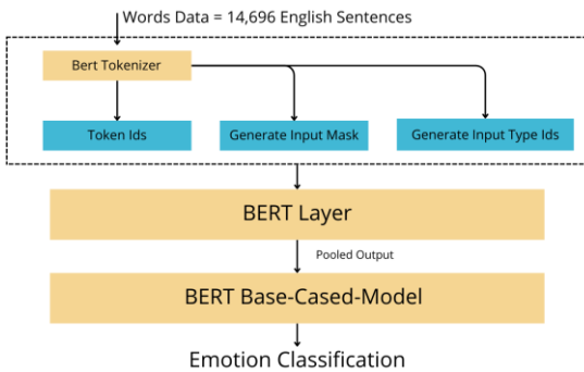
Figure 2. TER Proposed System Structure
