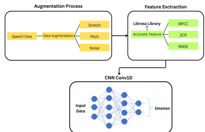
Figure 1. SER Proposed System Structure
