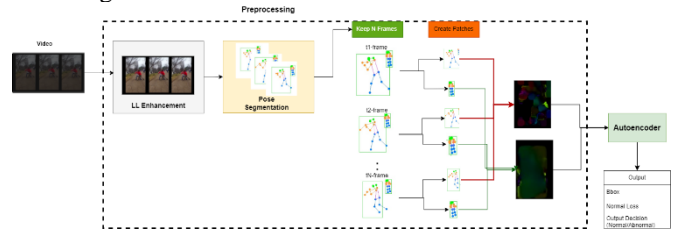
(Figure 2) Inference process of Our proposed Method
