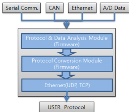
Fig. 2 The Structure of Communication Protocol Conversion
