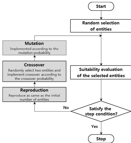
Figure 1. Process of Genetic Algorithms
