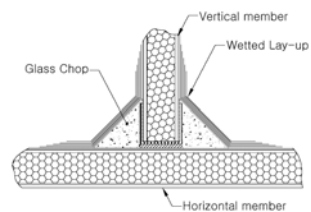
Fig 2. Schematic for Wetted Lay-up T-Joints
