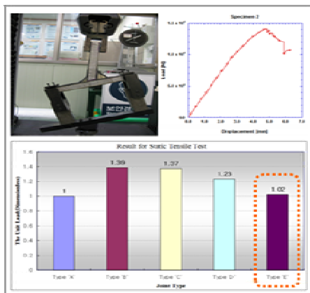
Fig 4. Test Schematic & Result for Tensile
