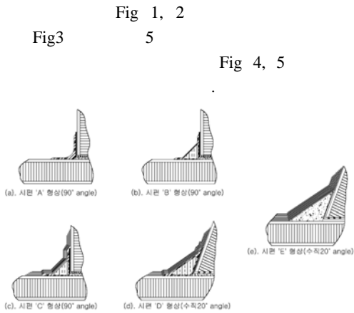
Fig 3. Structures for Test Specimen
