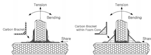
Fig 1. Features for general T-Joints
