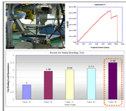
Fig 5. Test Schematic & Result for Bending
