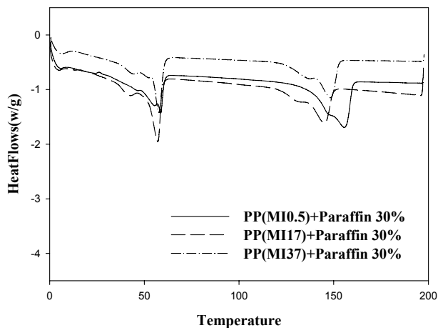
Fig. 1. DSC Thermo-diagrams of PP(MI0.5,17,37) and n -Paraffin 30%
