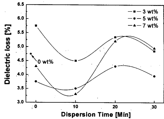
그림 3. Relative dielectric loss of Epoxy-Cloisite 30B specimens as a function of added clay amount.
