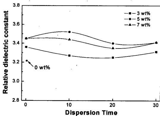
그림 2. Relative dielectric constant of Epoxy-Cloisite 30B specimens as a function of added clay amount.
