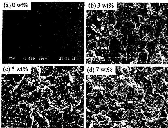
그림 1. SEM micrographs of epoxy-Cloisite 30B specimens as a function of added clay amount.
