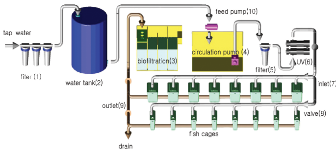
Fig. 2 Conceptual design of Zebra Auto System
