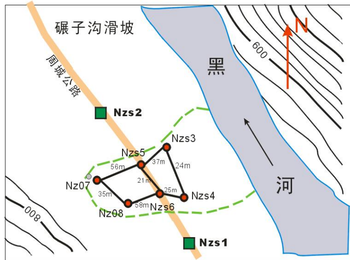
Figure 8. The monitored landslide over a reservoir
