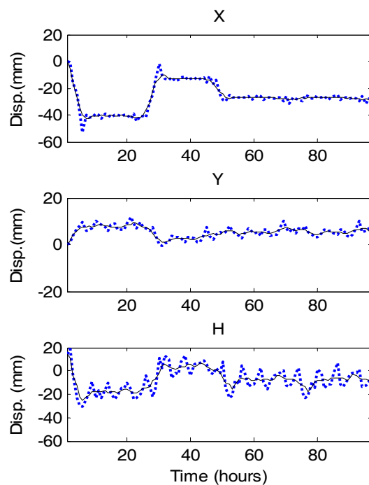
Figure 7. The measured displacement series
