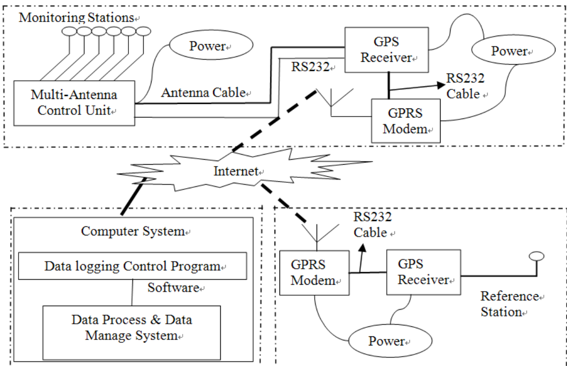
Figure 1. Multi-antenna GPS system structure
