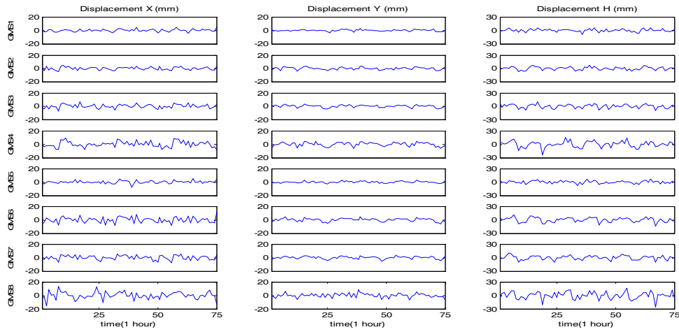
Figure 11. Displacement series with 1 hour data update interval
