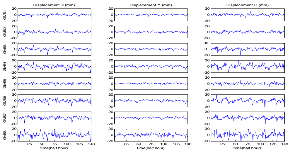
Figure 10. Displacement series in with 30 minute data update interval
