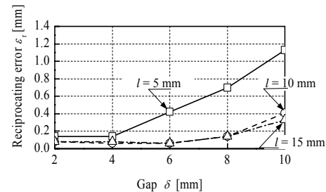
Fig. 2. Reciprocating error depending on the magnet size and gap.
