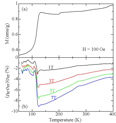
Fig. 1. (a) Magnetization and (b) Magnetoresistance vs T.
