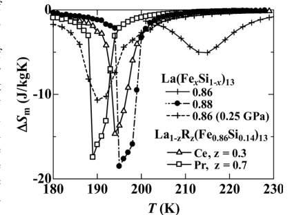
Fig. 1. Temperature dependence of \Delta S_m for \text{La}(\text{Fe}_x\text{Si}_{1-x})_{13} and \text{La}_{1-z}\text{R}_z(\text{Fe}_{0.86}\text{Si}_{0.14})_{13} .
