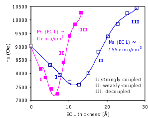
Fig. 1. Saturation field vs ECL thickness for different M_s values of ECL.
