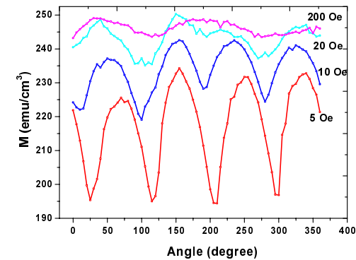
Fig. 1. Magnetization vs angle \phi of selected LSMO film at room temperature.
