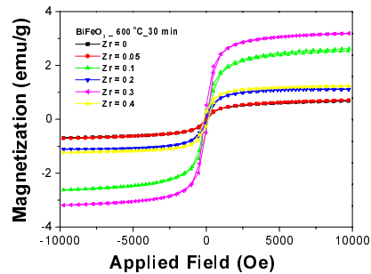
Fig. 1. The specific magnetizations of the BiFe 1-x Zr x O 3 ; x = 0, 0.1, 0.2, 0.3, 0.4 samples calcined in air for 30 min at 600°C, as a function of field, measured at 20°C.
