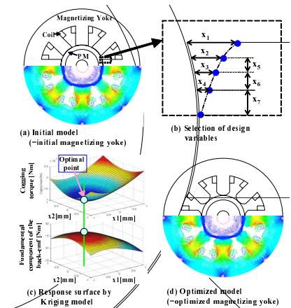
Fig. 1. Optimization of magnetizing yoke in PM motor.
