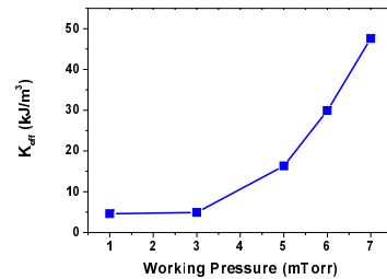
Fig. 1. The value of magnetic anisotropy of Tb(Fe 0.55 Co 0.45 ) 1.5 thin films as function of working pressure.
