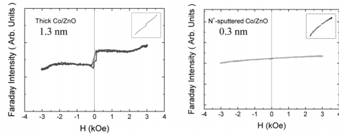
Fig. 2. the polar hysteresis loops of 1.3 nm Co/ZnO and N + -sputtered 0.3 nm Co/ZnO films.
