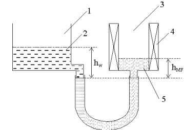
Fig. 1. Inductive magnetofluidic sensor.
