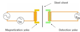
Fig. 1. Compose of magnetizing yoke and sensing yoke.
