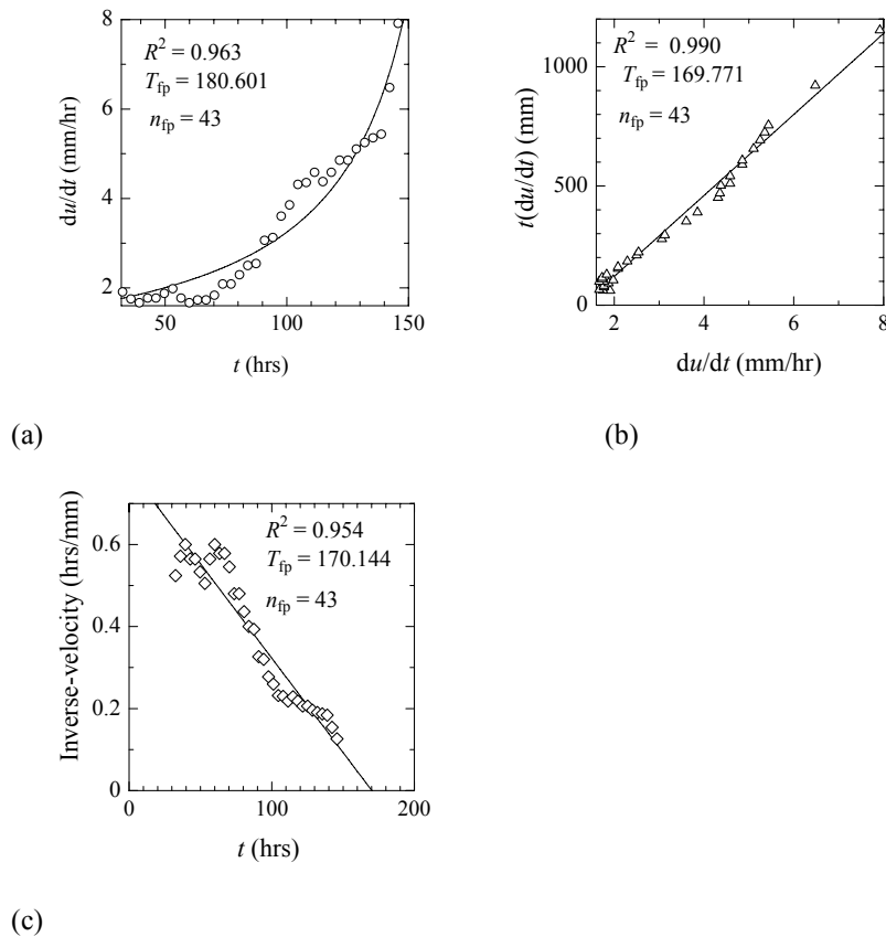
Fig. 2. Typical plots used for predictions of failure-time for Asamushi landslide using (a) NLA, (b) SLO and (c) INV method for all the data ( n_{ip} = 43 ). n_{ip} is the number of data.
