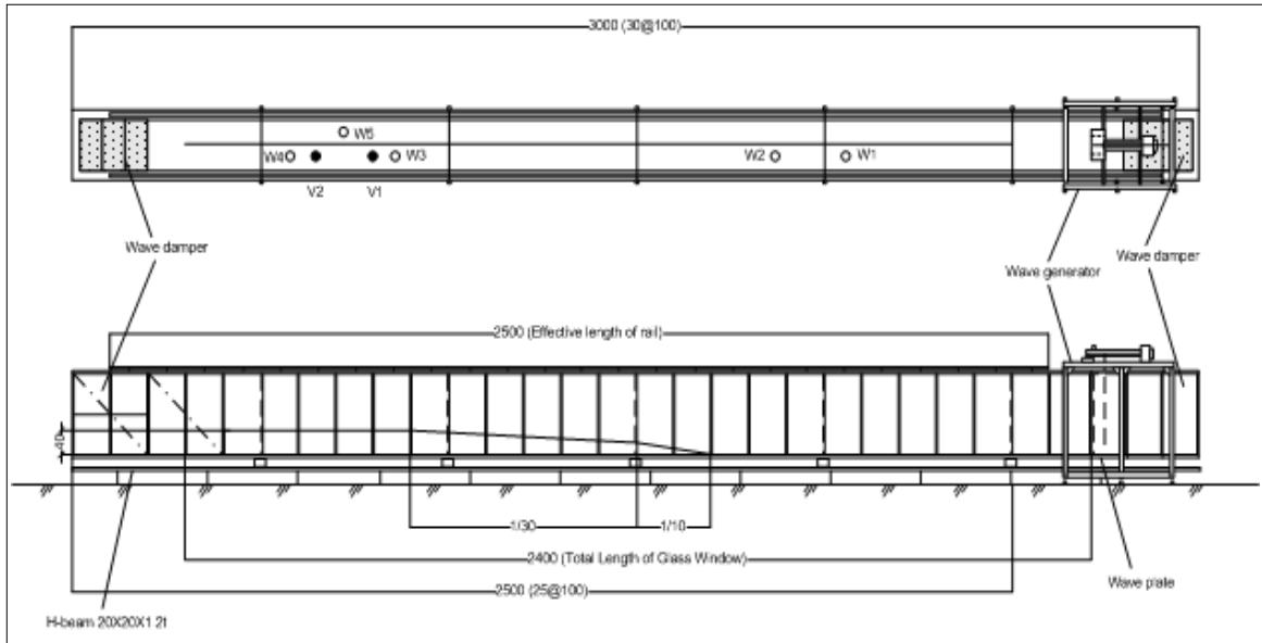
Fig. 1. Schematic section of Wave-Current 2-D
