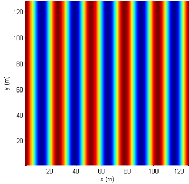
Fig. 2. Instantaneous surface elevation generated by Eq.(7) for surface current speed=14m/s.
