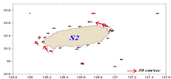
Fig. 8. Major amplitude axis and phase lag(deg.) of S2.
