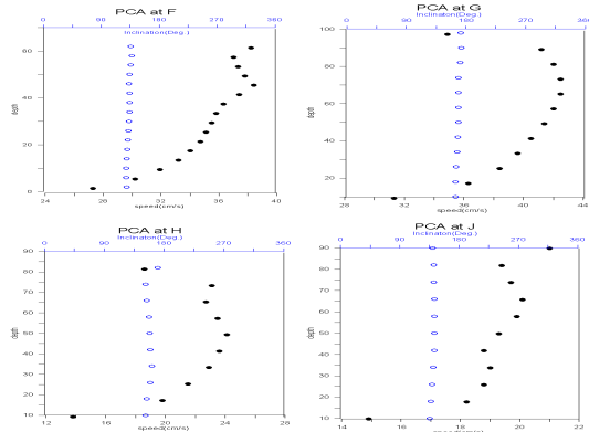
Fig. 11. Vertical variation of PCA Results.
