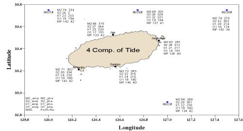
Fig. 3. Harmonic constants of Tide
