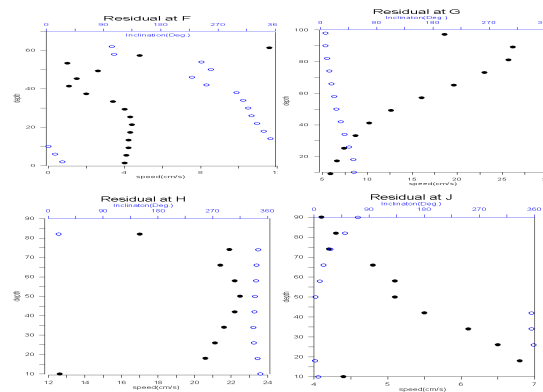
Fig. 12. Vertical variation of Residual Currents
