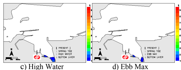
Fig. 8. Horizontal bottom temperature distributions during spring tide.
