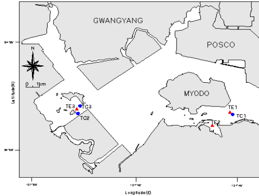
Fig.1. Observation stations of tidal current.
