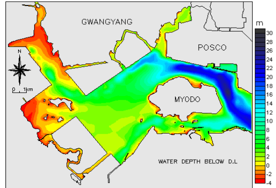
Fig. 4. Water depth below datum level.
