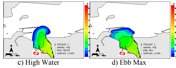
Fig. 6. Horizontal surface temperature distributions during spring tide.
