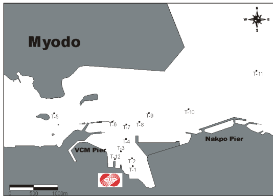
Fig. 2. Observation stations of temperature
