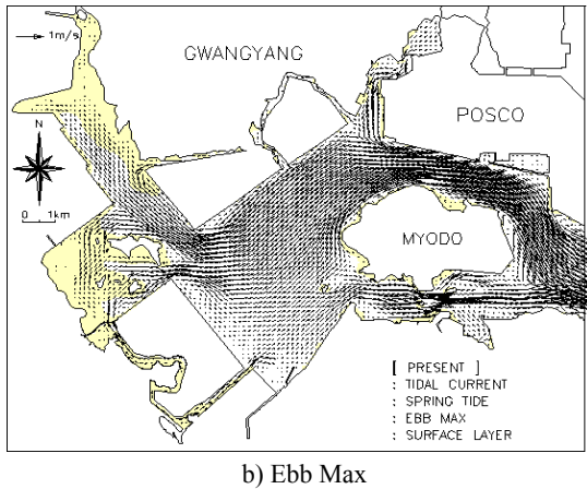
Fig. 5. Vector diagram of surface tidal currents during the spring tide.
