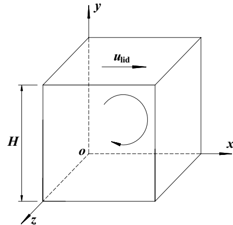
Fig. 2 Flow configuration of lid-driven cavity flow in a cubic cavity.
