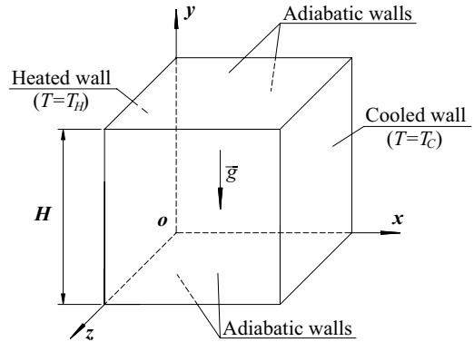
Fig. 18 Flow configuration of natural convection in a cubic cavity.
