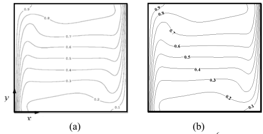
Fig. 19 Temperatures at the plane z=0.5H for Ra=10^6 , obtained (a) from reference[35], (b) by IDEAL algorithm.
