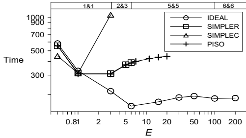
(a) Re=100
