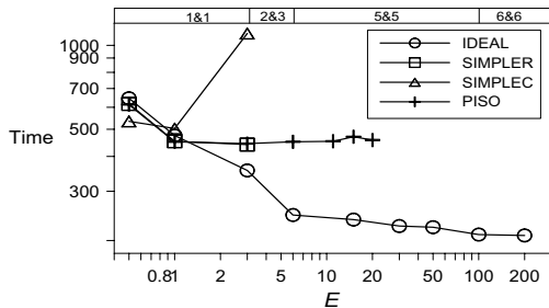
(b) Re=300
