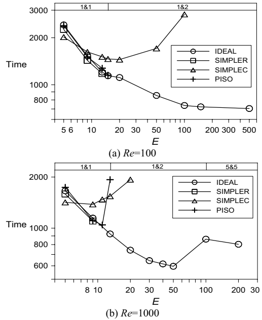
Fig. 6 Comparison of computation time and robustness of IDEAL, SIMPLER, SIMPLEC and PISO algorithms for (a) Re=100 and (b) Re=1000 with grid number= 82 \times 82 \times 82 of problem 1.
