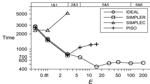
(a) Re=100
