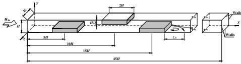
Fig. 15 Flow configuration of laminar fluid flow through a duct with complicated structure.
