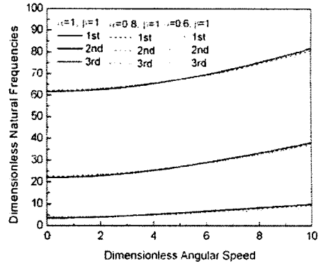
Fig. 5 Natural frequency variation vs. angular Speed ( \delta = 0.5 )
