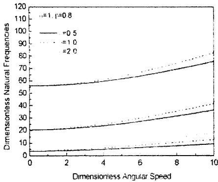
Fig. 6 Natural frequency variation vs. angular Speed
