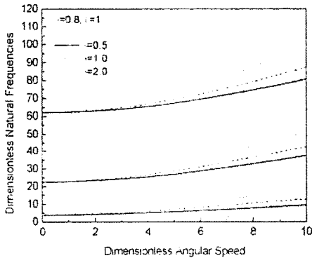
Fig. 7 Natural frequency variation vs. angular Speed
