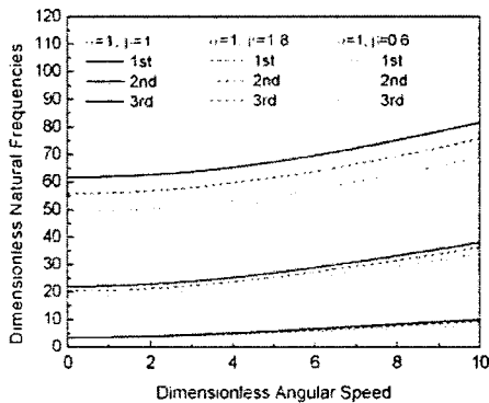
Fig. 4 Natural frequency variation vs. angular Speed ( \delta = 0.5 )
