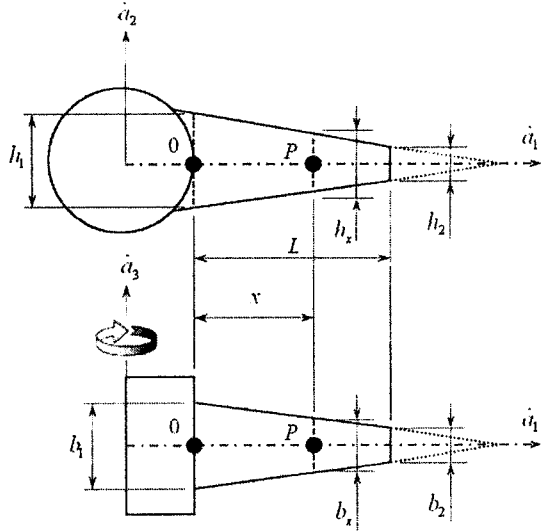
Fig. 2 A cantilever beam with tapered cross section
