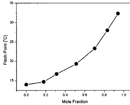
Fig. 3. The result of flash point for water - ethanol system.
