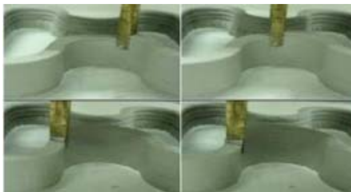
<Figure 9> Sequence of the process showing the effect of the short side trowel in fabricating concave corners
