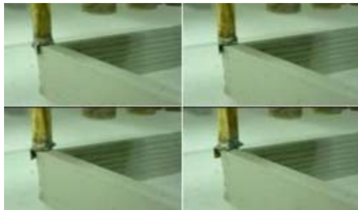
<Figure 5> Sequence of the process showing the effect of the long side trowel when fabricating sharp square corners
