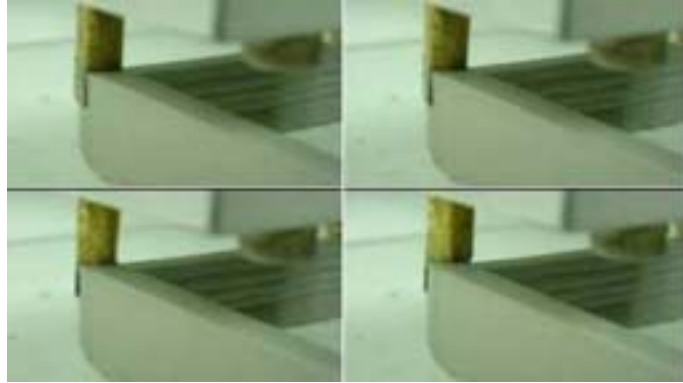
<Figure 8>. Sequence of the process showing the effect of short side trowel in fabricating sharp square corners
