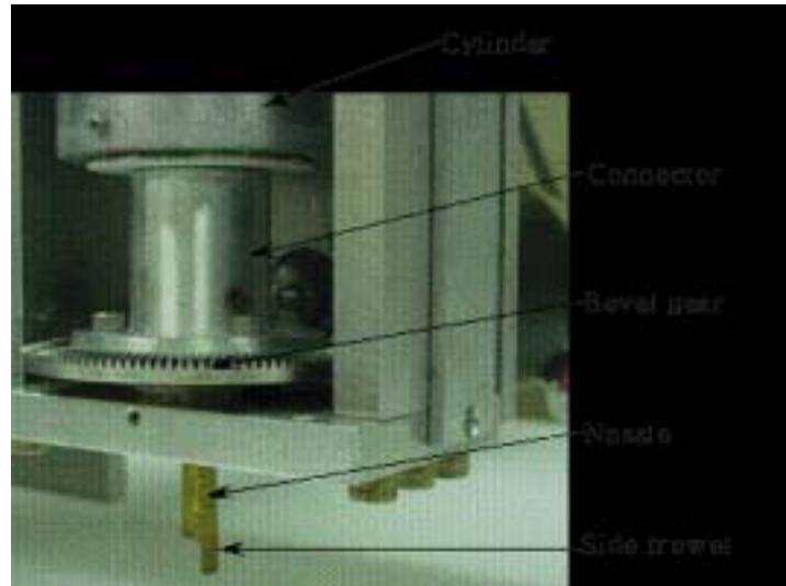
<Figure 3> Trowel rotation system of CC process
