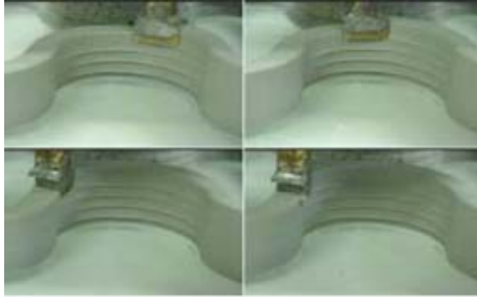
<Figure 6> Sequence of the process showing the effect of the long side trowel in fabricating concave corners
