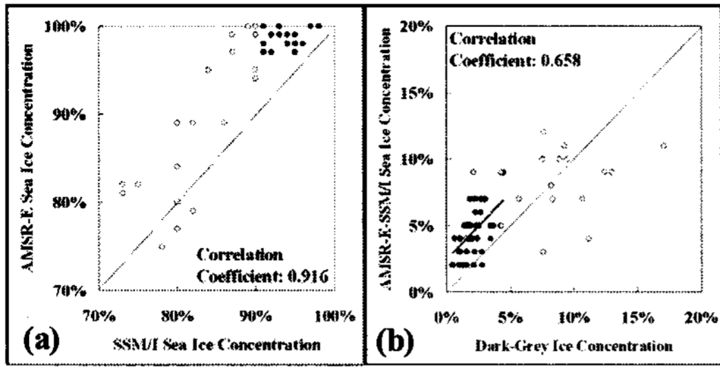
Figure 3. (a) The relationship between SSM/I and AMSR-E sea ice concentration, (b) The relationship between EOC D and AMSR-E sea ice concentration.
