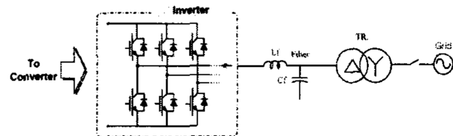
Fig 4. DC-AC Inverter, Transformer, 계통배전반.
