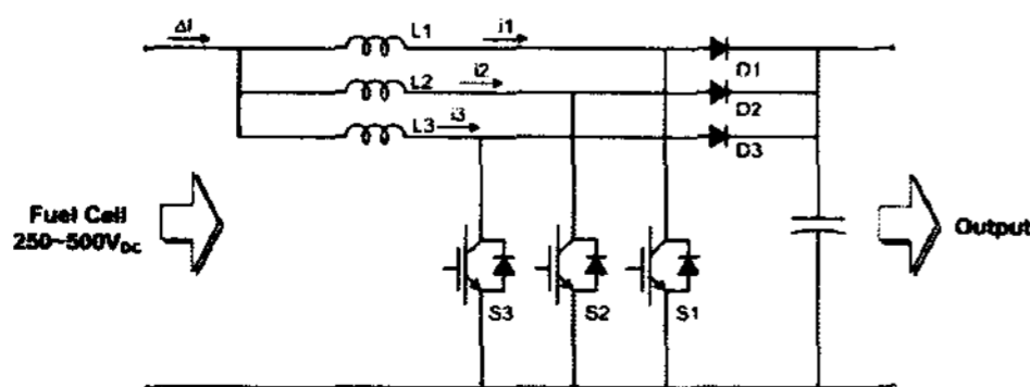
Fig 2. Interleaved Boost Converter
