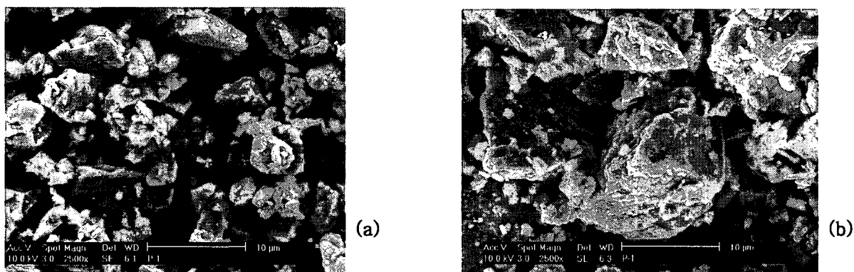
Fig. 2. SEM micrographs for the sample \text{CaAl}_2\text{O}_4:\text{Eu}^{2+}
