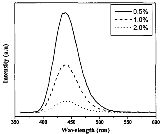
Fig. 4. Emission spectra for \text{CaAl}_2\text{O}_4:\text{Eu}^{2+}
