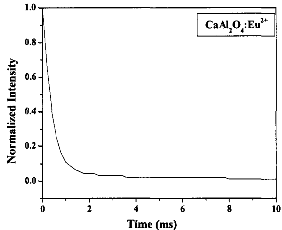
Fig. 5. Decay time for \text{CaAl}_2\text{O}_4:\text{Eu}^{2+}
