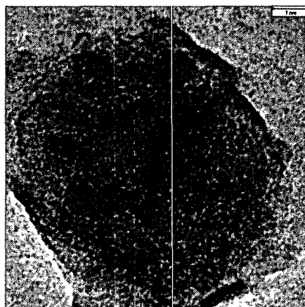
Fig. 3. TEM micrographs for the sample \text{CaAl}_2\text{O}_4:\text{Eu}^{2+}
