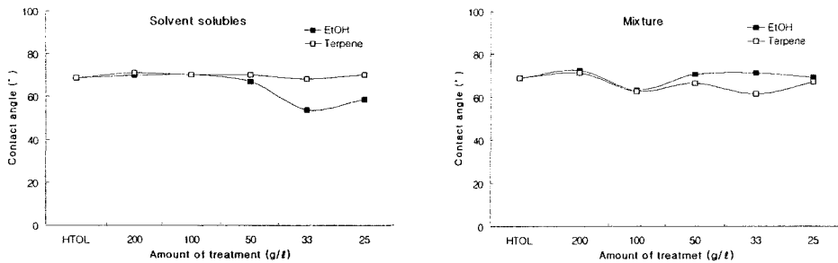
Figure 5. Contact angle of Hanji treated with oriental lacquer.
