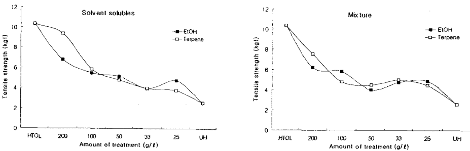
Figure 2. Tensile strength of Hanji treated with oriental lacquer.
