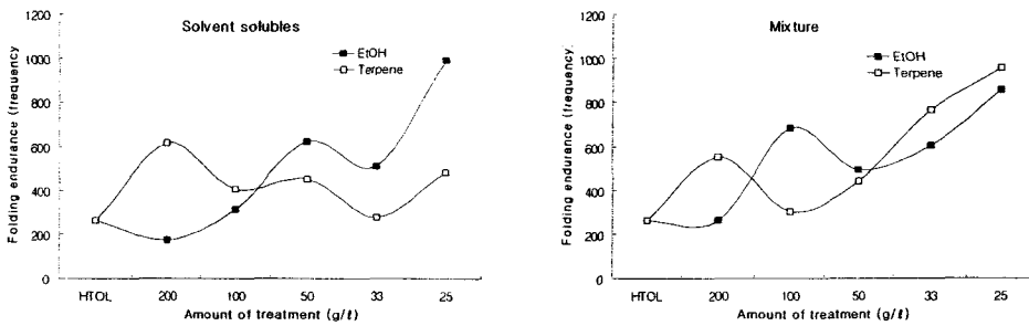
Figure 3. Folding endurance of Hanji treated with oriental lacpuer.
