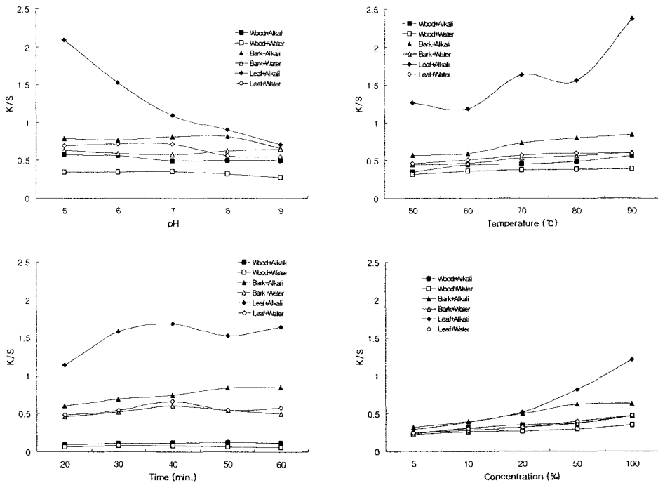
Figure 1. K/S values Hanji dyed with N. sericea Koidz extract by conditions.
