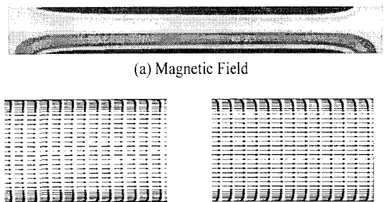
(b) Velocity Profile with EMBR (c) Velocity Profile without EMBR
