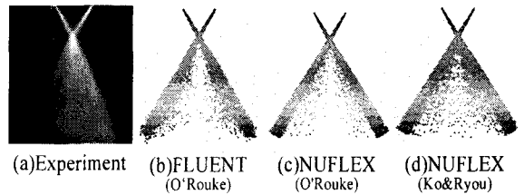
Fig. 6 Validation of spray collision models
