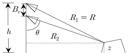
Fig. 1. InSAR configuration.
