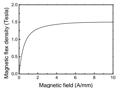
Fig. 3 The B-H curve of the low carbon steel (S20C)
