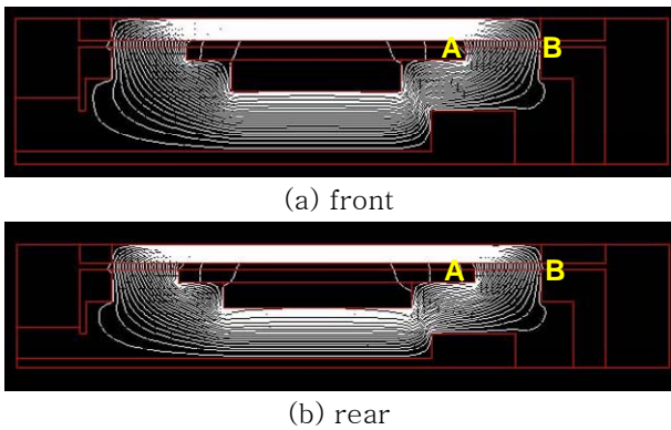
Fig. 7 2D magnetic flux lines of the optimized MR shock absorbers
