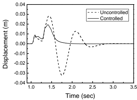
Fig. 11 Bump responses of the full-vehicle
