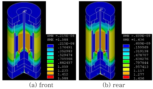
Fig. 6 3D magnetic flux densities of the optimized MR shock absorbers
