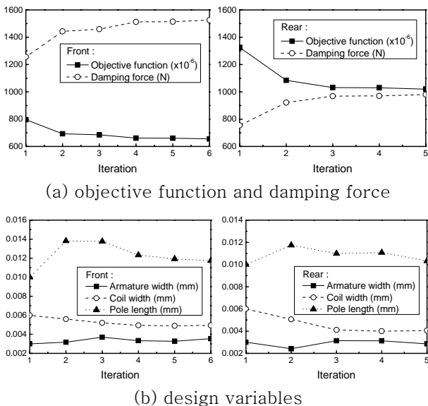
Fig. 5 Optimization results of the MR shock absorbers
