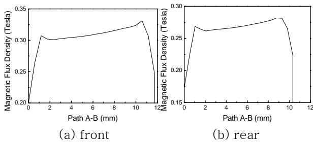
Fig. 8 Magnetic flux densities of magnetic poles along path A-B
