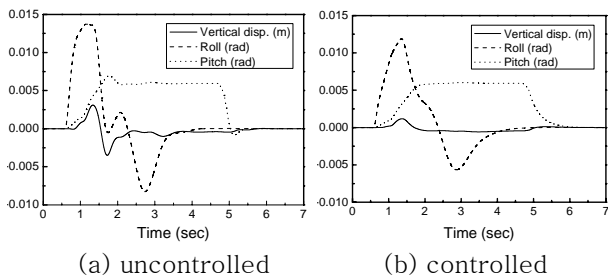
Fig. 12 Obstacle avoidance responses of the full-vehicle
