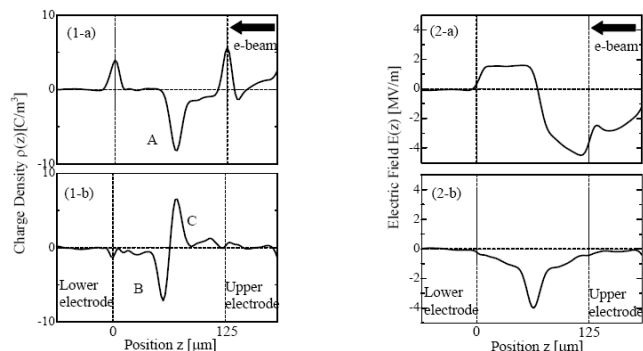
Fig. 1. Charge (1) and electric field (2) distributions in e-beam irradiated polyimide film for (a) 10, (b) 600s, respectively.
