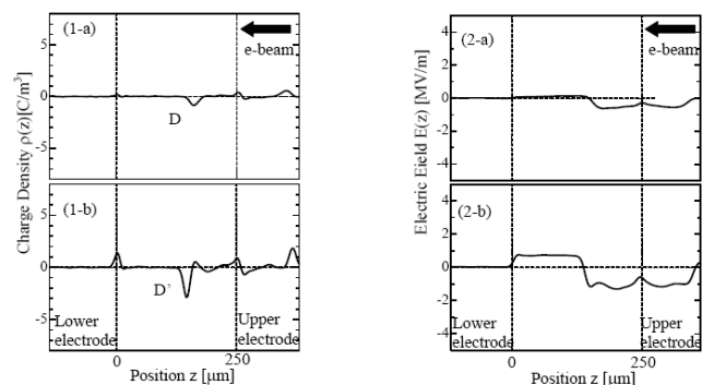
Fig. 2. Charge (1) and electric field (2) distributions in e-beam irradiated polystyrene film for (a) 10, (b) 600s, respectively.
